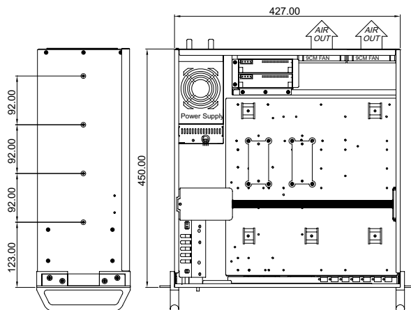
Left-side View
